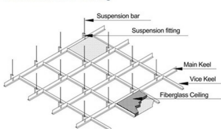
Installation for ceiling
